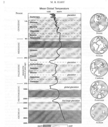
Fig. 1. Generalized temperature history of the planet (adapted from Merritts et al. 1998).
